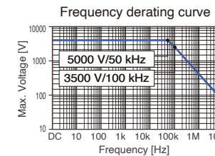
AC/DC HIGH VOLTAGE DIVIDER VT1005
