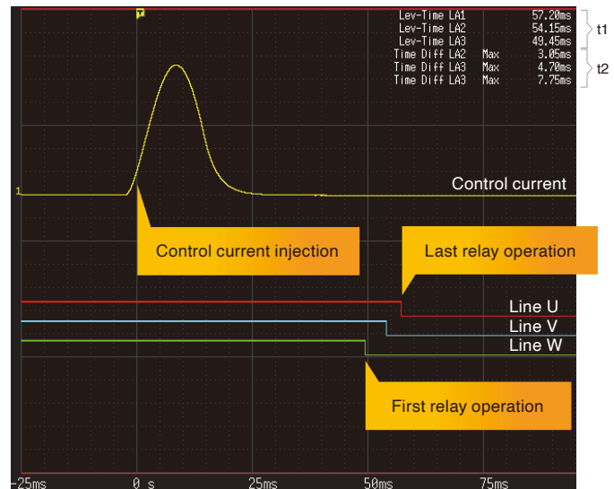
t1 < Specified time from control current injection to relay opening/closing t2 < Specified time difference between each contact
