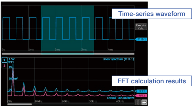
Time sequence + FFT screen
