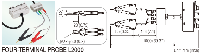
FOUR-TERMINAL PROBE L2000 Cable length 1 m (3.28 ft), DC to 8 MHz, impedance characteristics of 50 Ω, 4-terminal pair configuration, measurable conductor diameter: \phi 0.3 (0.01 in.) to 5 mm (0.20 in.)
