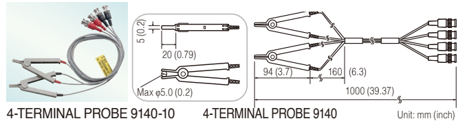
4-TERMINAL PROBE 9140-10 Cable length 1 m (3.28 ft), DC to 200 kHz, impedance characteristics of 50 Ω, 4-terminal pair configuration, measurable conductor diameter: \phi 0.3 (0.01 in.) to 5 mm (0.20 in.)
