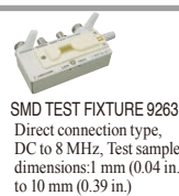
TEST FIXTURE 9262 Direct connection type, DC to 8 MHz, measurable conductor diameter: \phi 0.3 (0.01 in.) to 2 mm (0.08 in.)
