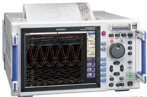
MR8827 main unit with U8350 Printer Unit installed
