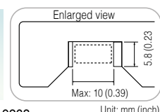
SMD TEST FIXTURE 9263 Direct connection type, DC to 8 MHz, Test sample dimensions: 1 mm (0.04 in.) to 10 mm (0.39 in.)
