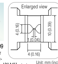
SMD TEST FIXTURE 9677 Direct connection type, For measuring SMDs with electrodes on the side; DC to 120 MHz, test sample dimensions: 3.5 mm \pm 0.5 mm (0.14 in. \pm 0.02 in.)
