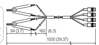
4-TERMINAL PROBE 9140 Cable length 1 m (3.28 ft), DC to 100 kHz, impedance characteristics of 75 Ω, 4-terminal configuration, measurable conductor diameter: \phi 0.3 (0.01 in.) to 5 mm (0.20 in.)
