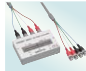
TEST FIXTURE 9261-10 Cable length 1 m (3.28 ft), DC to 8 MHz, impedance characteristics of 50 Ω, 4-terminal pair configuration, measurable conductor diameter: \phi 0.3 (0.01 in.) to 1.5 mm (0.06 in.)
