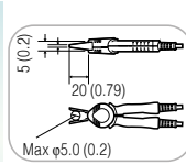
FOUR-TERMINAL PROBE L2000 Cable length 1 m (3.28 ft), DC to 8 MHz, impedance characteristics of 50 Ω, 4-terminal pair configuration, measurable conductor diameter: \phi 0.3 (0.01 in.) to 5 mm (0.20 in.)
