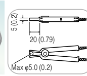
4-TERMINAL PROBE 9140-10 Cable length 1 m (3.28 ft), DC to 200 kHz, impedance characteristics of 50 Ω, 4-terminal pair configuration, measurable conductor diameter: \phi 0.3 (0.01 in.) to 5 mm (0.20 in.)
