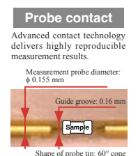
SMD TEST FIXTURE IM9110 Direct connection two-terminal measurement type for measuring SMDs, DC to 1 MHz, measurable sample sizes: 008004 (inch)
