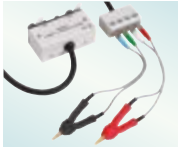
FOUR-TERMINAL PROBE L2000 Cable length 1 m (3.28 ft), DC to 8 MHz, impedance characteristics of 50 Ω, 4-terminal pair configuration, measurable conductor diameter: \phi 0.3 (0.01 in.) to 5 mm (0.20 in.)
