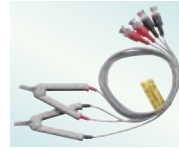
4-TERMINAL PROBE 9140-10 Cable length 1 m (3.28 ft), DC to 200 kHz, impedance characteristics of 50 Ω, 4-terminal pair configuration, measurable conductor diameter: \phi 0.3 (0.01 in.) to 5 mm (0.20 in.)
