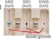
SMD TEST FIXTURE IM9100 Direct connection type, SMDs with electrodes on the bottom, DC to 8 MHz, metric(inch): 0402(01005), 0603(0201), 1005(0402)
