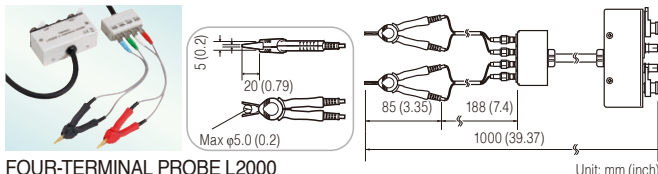
FOUR-TERMINAL PROBE L2000 Cable length 1 m (3.28 ft), DC to 8 MHz, impedance characteristics of 50 Ω, 4-terminal pair configuration, measurable conductor diameter: φ0.3 (0.01 in.) to 5 mm (0.20 in.)
