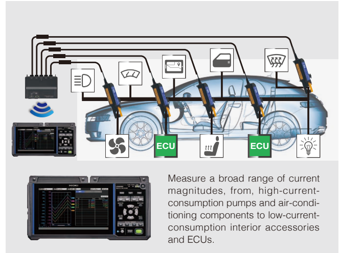
WIRELESS CURRENT MODULE LR8536
